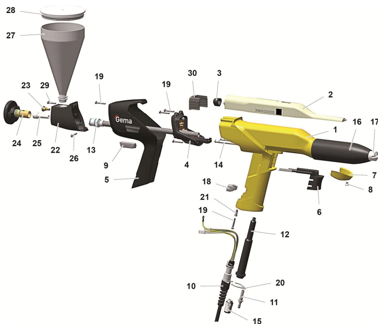
fig. 10: OptiSelect Pro GM04-CF – spare parts
