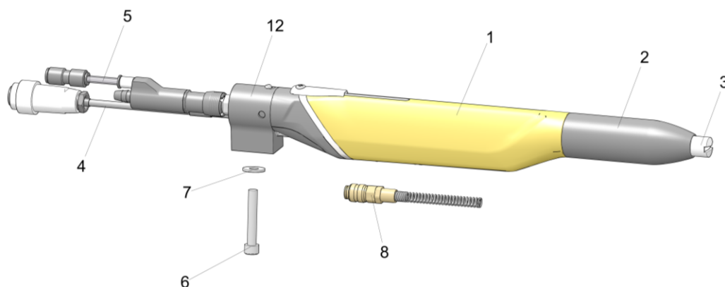
OptiGun GA03-P – complete
