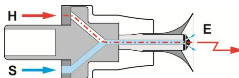
Round jet nozzle with vented deflector and vented central electrode
