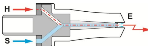
Flat jet nozzle with vented central electrode
