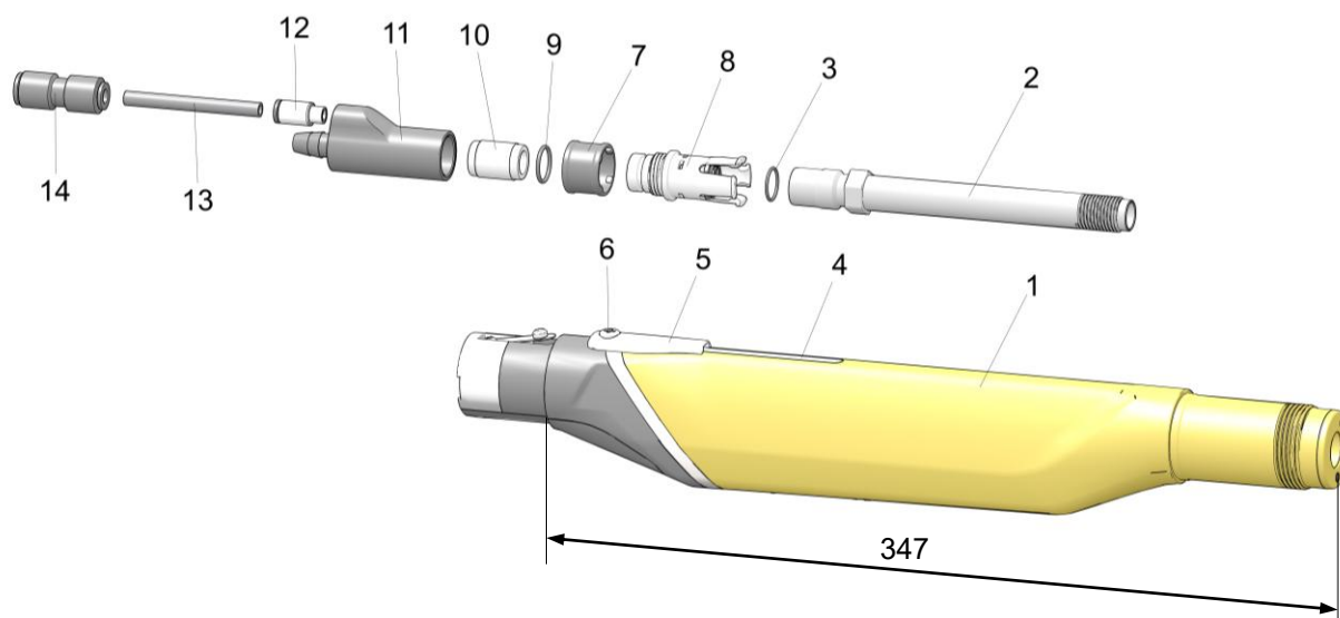
OptiGun GA03-P – gun body
