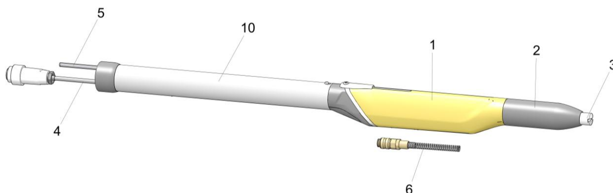
OptiGun GA03-P-X – complete
