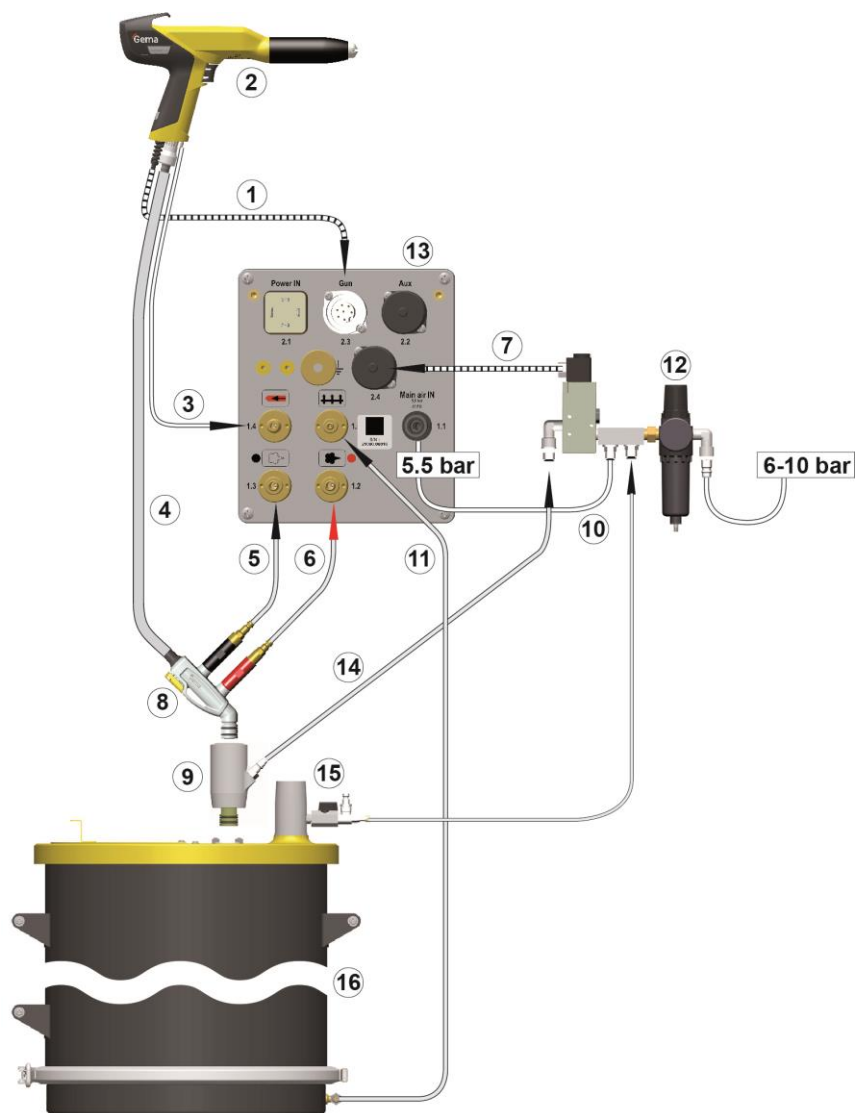
fig. 7: Connecting guide – overview
