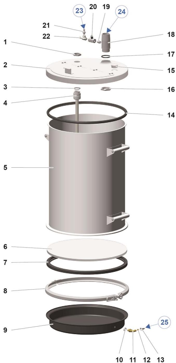
fig. 11: HF05-50 Powder Hopper
