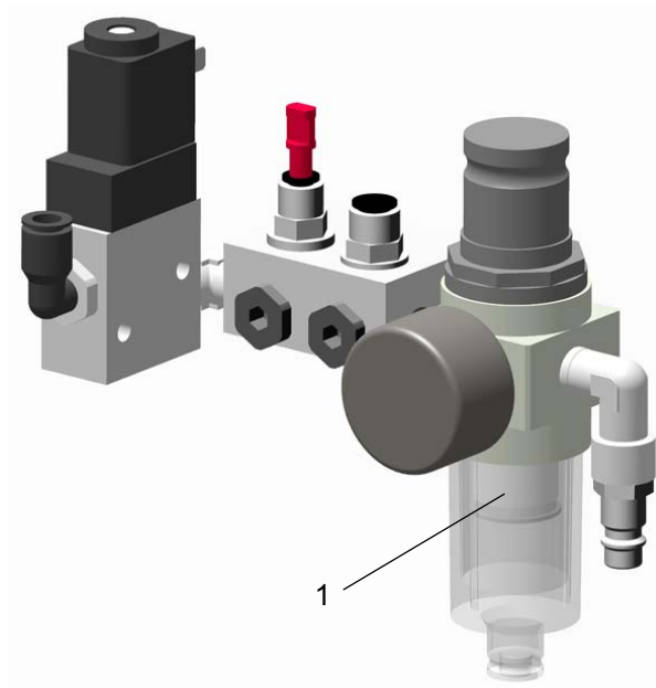
OptiFlex 2 L - Pneumatic group
