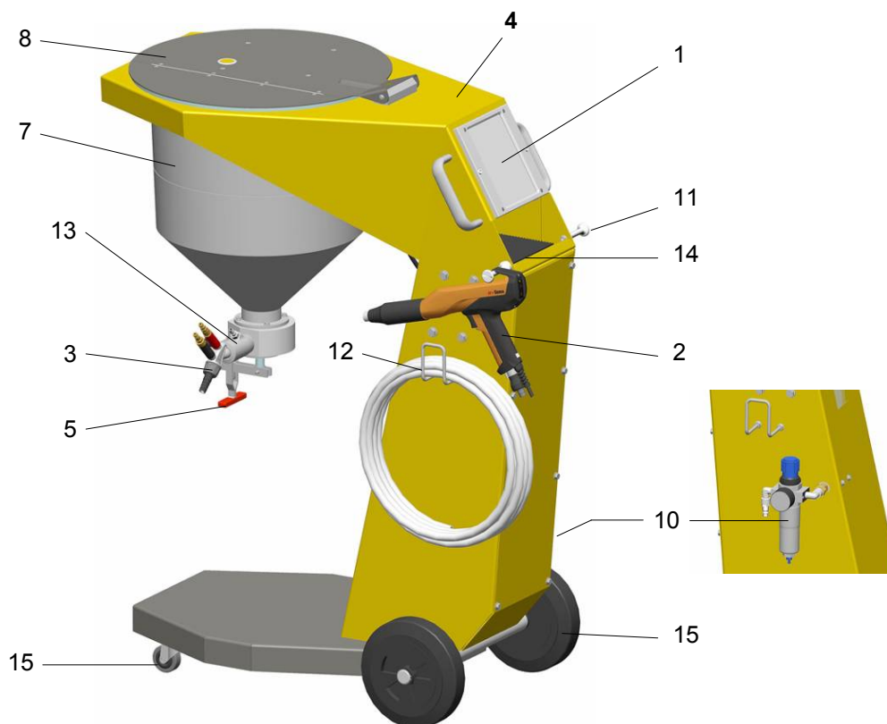
OptiFlex 2 S manual coating equipment - Structure
